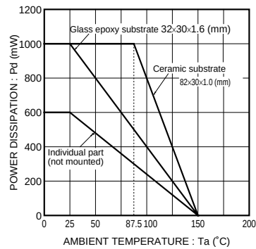
Fig.1 Derating curve
