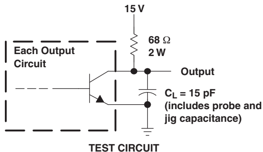
Figure 3. Common-Emitter Configuration
