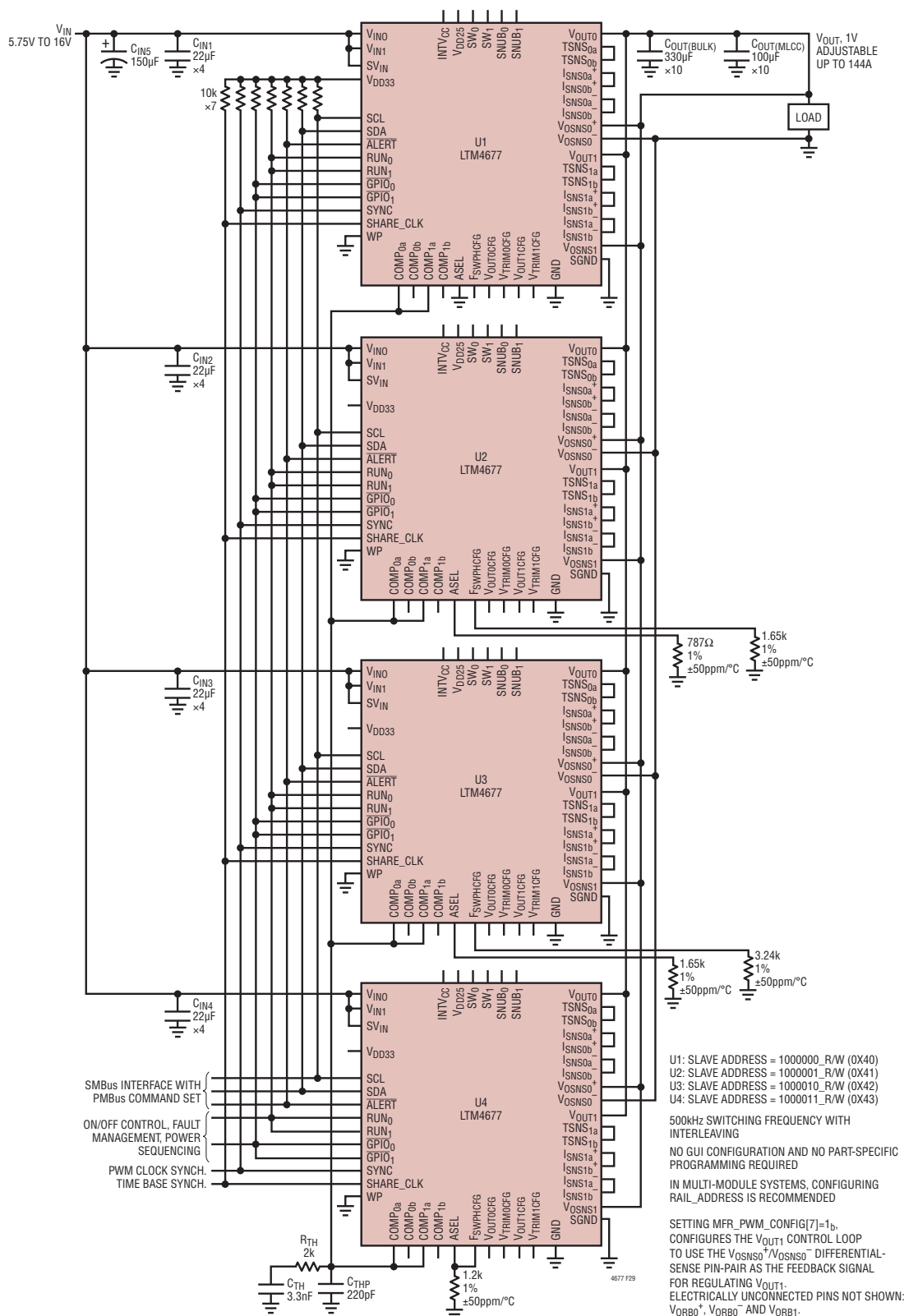
Figure 29. Four Paralleled LTM4677 Producing 1V OUT at Up to 144A. Integrated Power System Management Features Accessible Over 2-Wire I 2 C/SMBus/PMBus Serial Interface. For Evaluation and More Information, See Demo Boards DC2143
