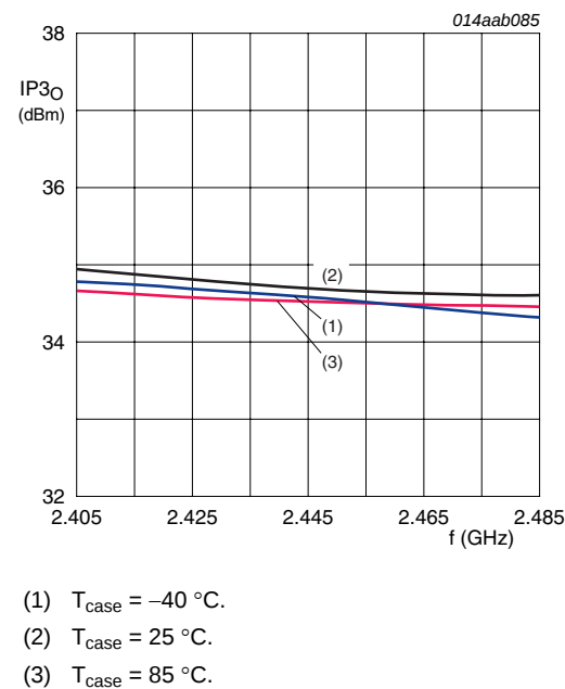
Fig 39. Output third-order intercept point as a function of frequency
