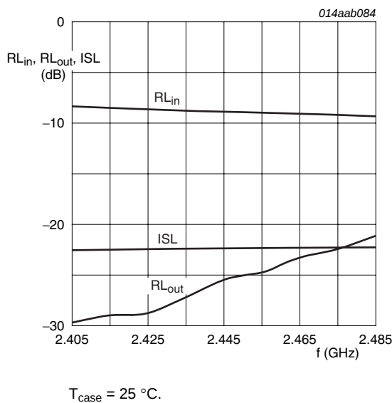
Fig 38. Input return loss, output return loss and isolation as a function of frequency
