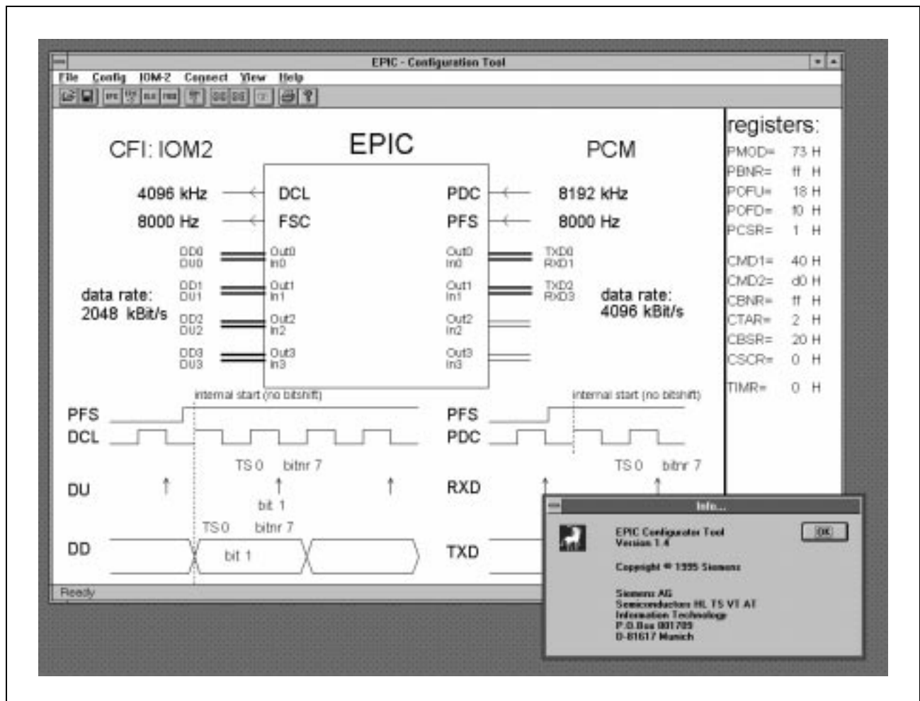
Figure 107 EPIC® Configuration Tool: Screen Shot
