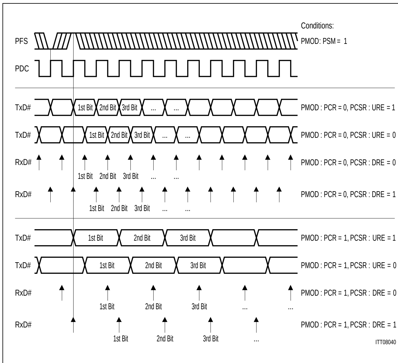
Figure 25 PCM Interface Framing for PMOD:PSM = 1
