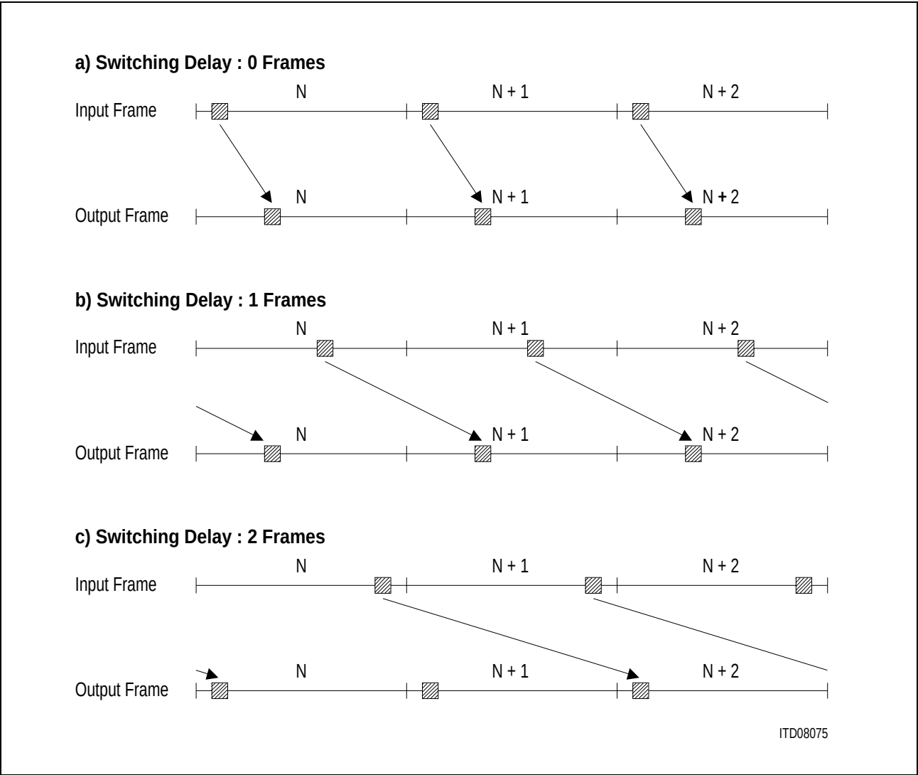
Figure 60 Switching Delays
