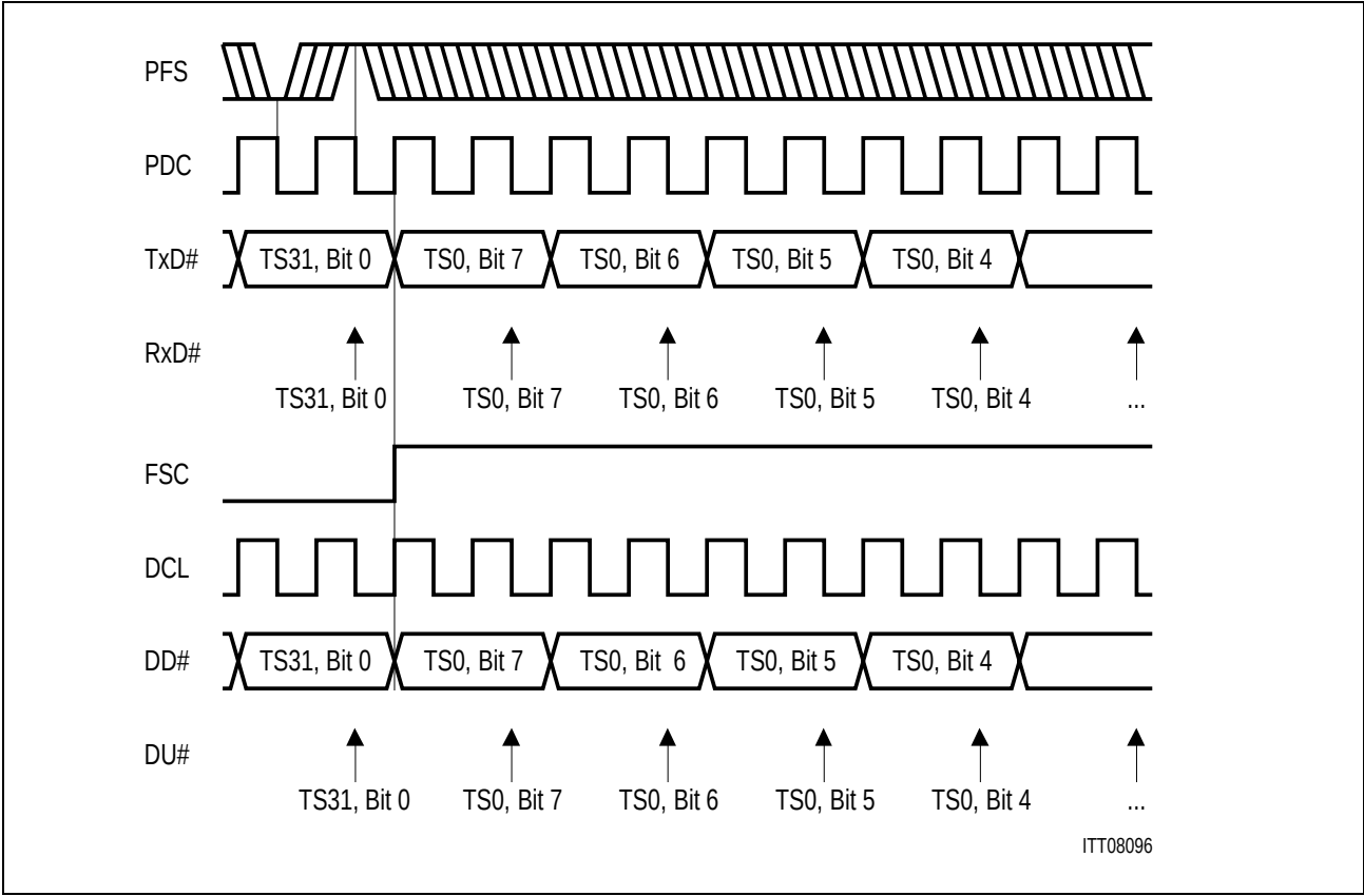
Figure 80 Typical IOM ® -2 Line Card Timing
