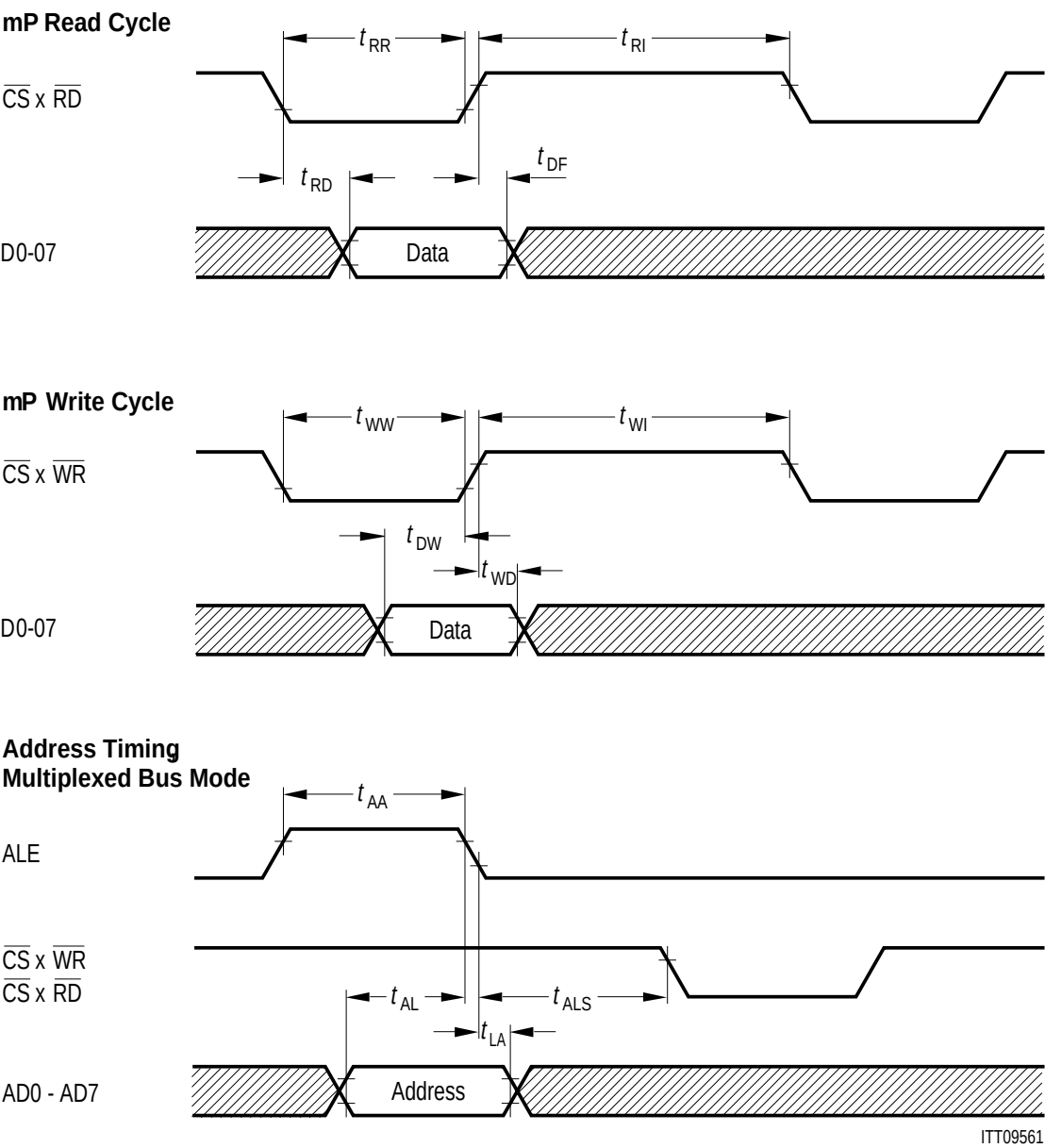
Figure 90 Siemens/Intel Bus Mode
