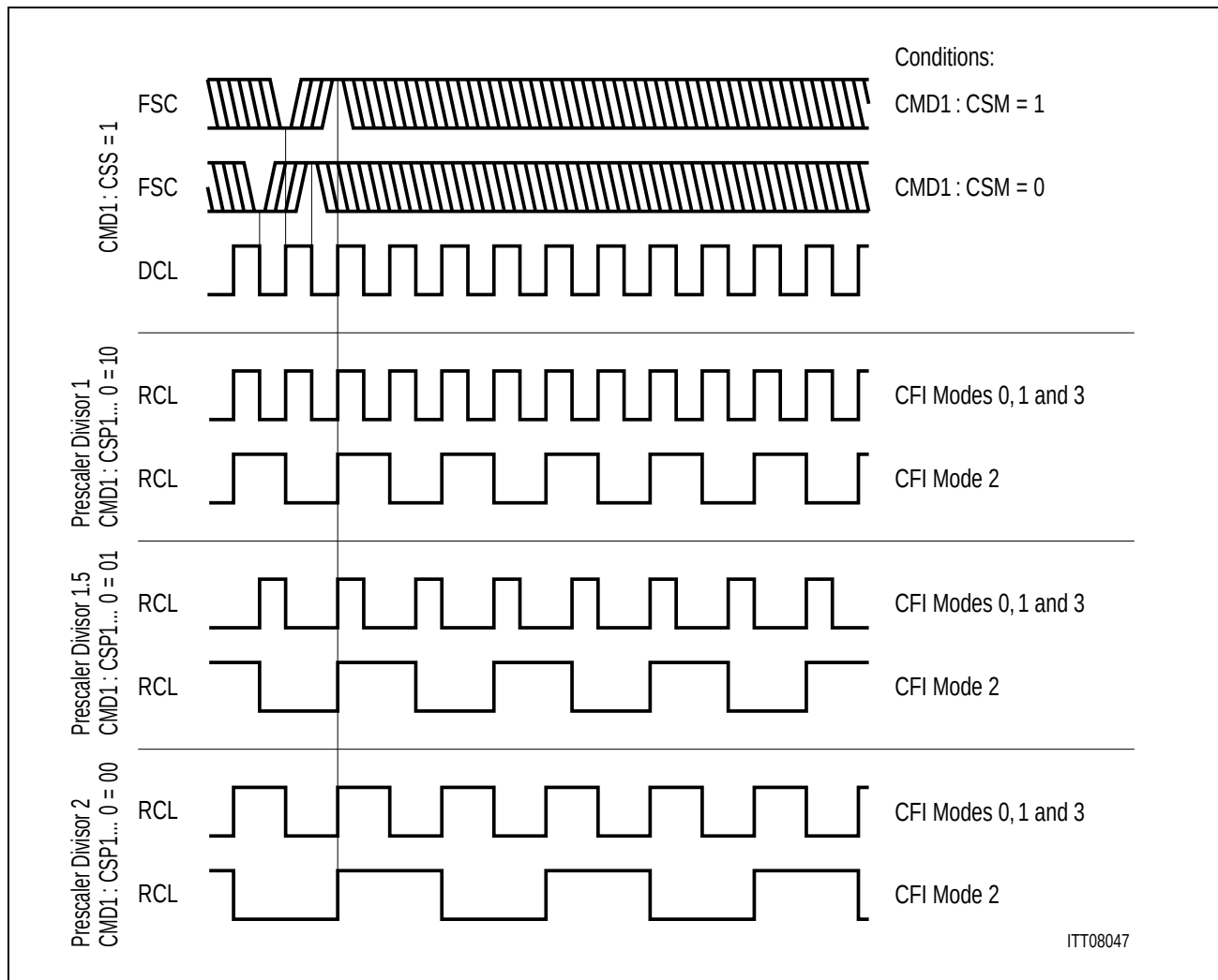
Figure 32 Clock Signal Timing for the Different Prescaler Divisors if \text{CMD1:CSS} = 1
