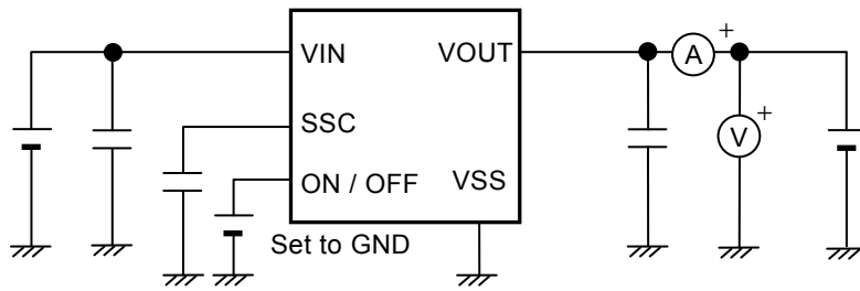
Figure 8 Test Circuit 6
