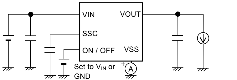
Figure 4 Test Circuit 2
