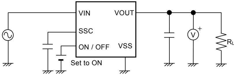
Figure 7 Test Circuit 5
