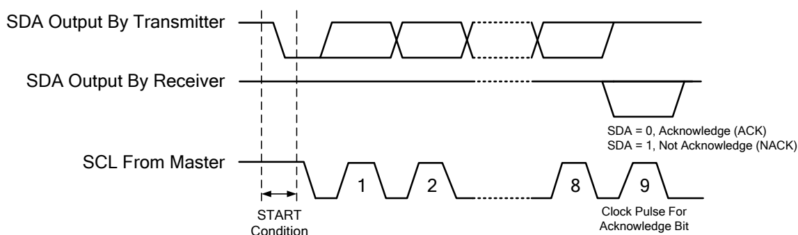
Figure 15-5. Acknowledge Bit
