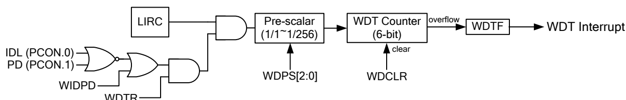
Figure 12-2. Watchdog Timer Block Diagram
