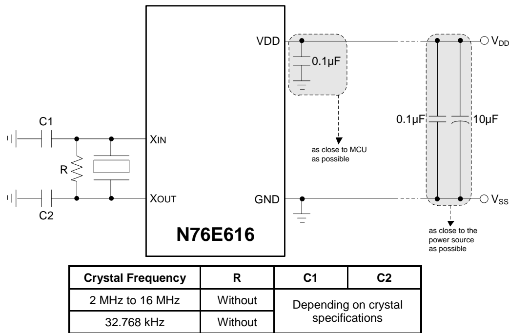
Figure 4-2. Application Circuit with External Crystal
