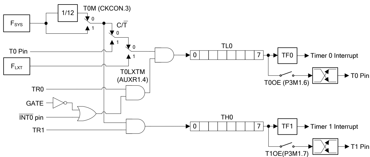
Figure 9-4. Timer/Counter 0 in Mode 3
