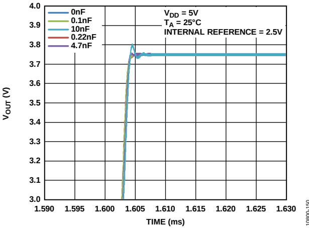
Figure 41. Settling Time vs. Capacitive Load
