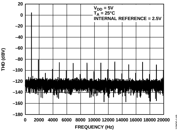
Figure 40. Total Harmonic Distortion @ 1 kHz
