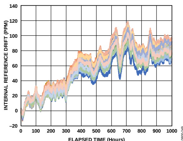
Figure 49. Reference Drift Through to 1000 Hours
