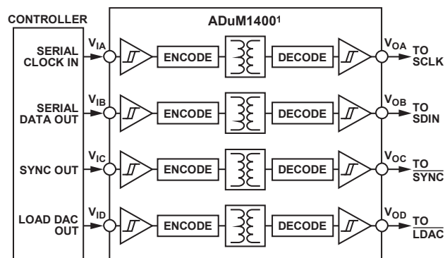
Figure 54. Isolated Interface
