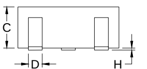
3-Lead SOT-23 Plastic Surface Mounted Package HSMC Package Code: N
