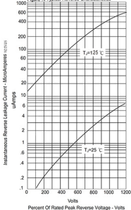
Figure 4-Typical Reverse Characteristics
