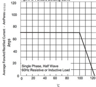
Figure 2-Forward Derating Curve
