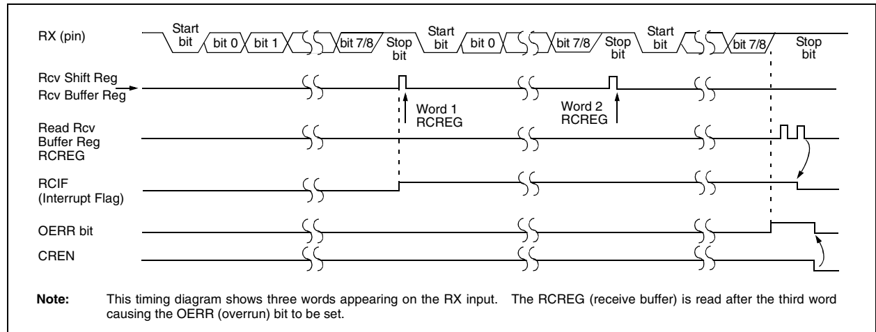
FIGURE 18-7: ASYNCHRONOUS RECEPTION
