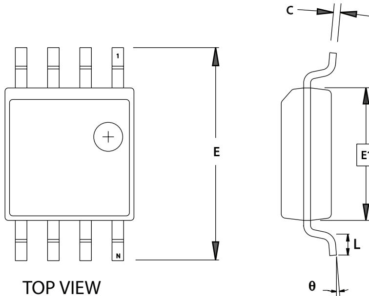
END VIEW
