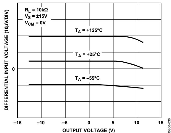
Figure 30. Open-Loop Linearity of the OP297
