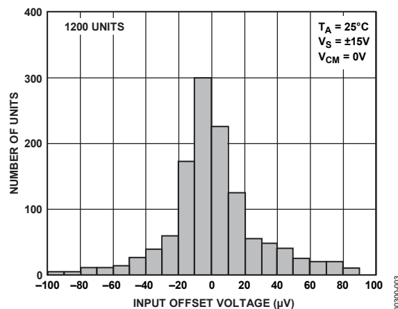
Figure 3. Very Low Offset
