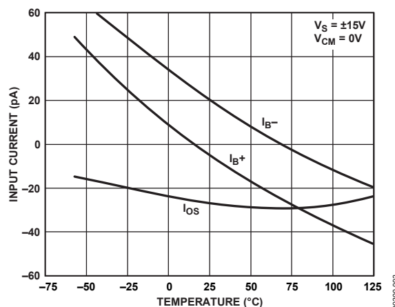
Figure 2. Low Bias Current over Temperature
