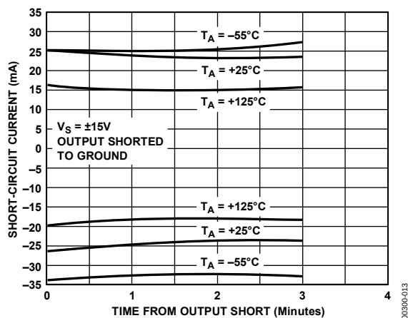
Figure 13. Short-Circuit Current vs. Time, Temperature
