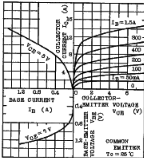
STATIC CHARACTERISTICS
