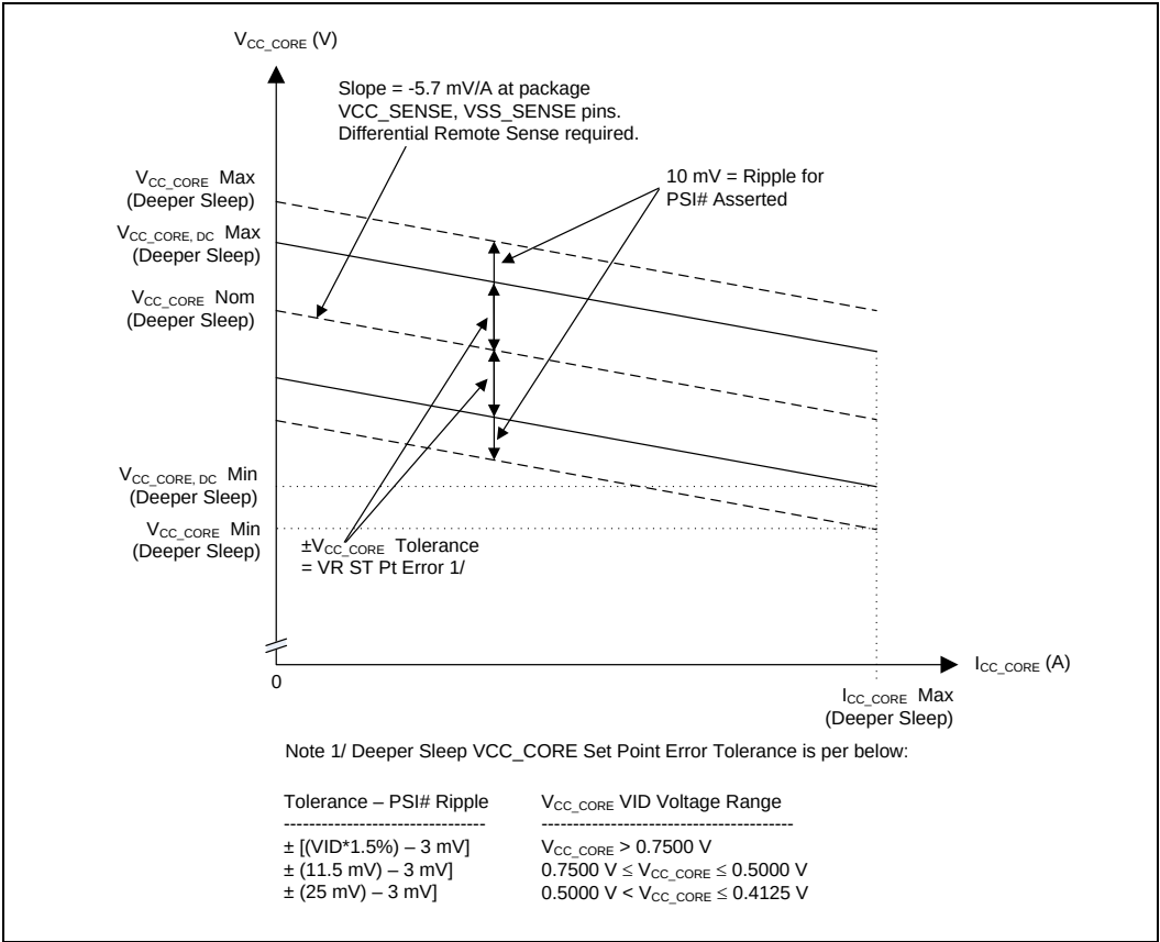
Figure 7. Deeper Sleep V_{CC} and I_{CC} Loadline
