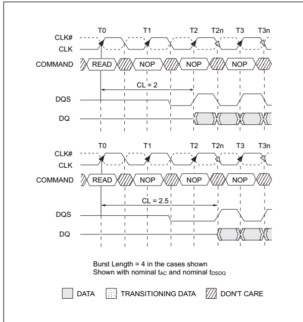
FIGURE 4 – CAS LATENCY
