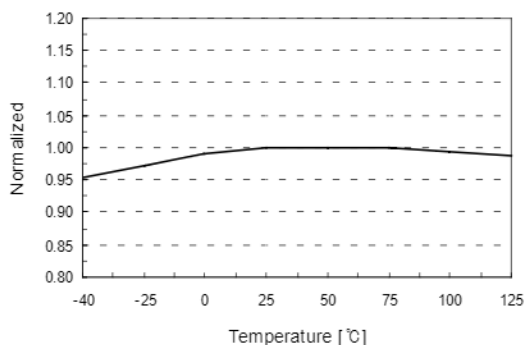
Figure 4. Operating Frequency ( f_{\text{OSC}} ) vs. T_A
