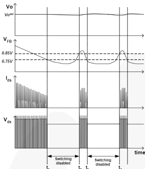
Figure 18. Burst-Mode Operation
