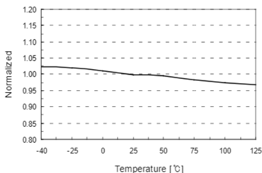
Figure 8. Shutdown Feedback Voltage ( V_{\text{SD}} ) vs. T_A
