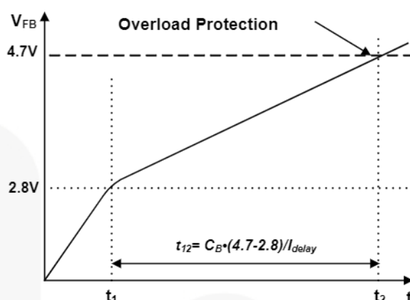
Figure 17. Overload Protection
