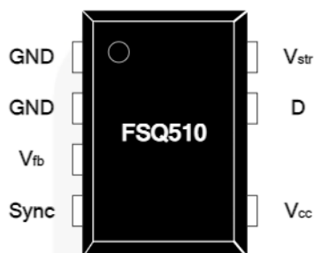
Figure 3. Pin Assignments
