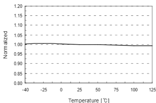
Figure 9. Maximum Duty Cycle ( D_{\text{MAX}} ) vs. T_A
