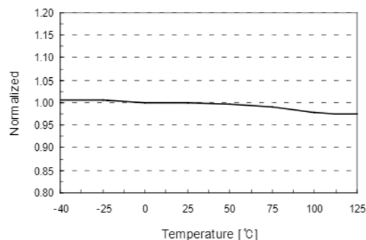
Figure 5. Peak Current Limit ( I_{\text{LIM}} ) vs. T_A
