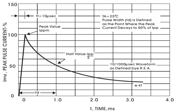
FIGURE 3-PULSE WAVEFORM
