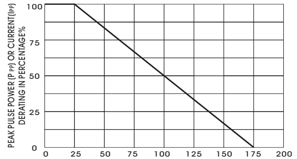
FIGURE 2-PULSE DERATING CURVE
