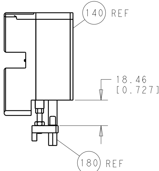
HOLDDOWN SET-UP
