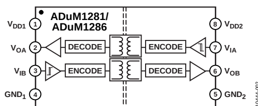
图2. ADuM1281/ADuM1286
