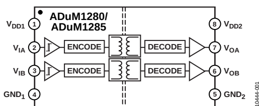
图1. ADuM1280/ADuM1285
