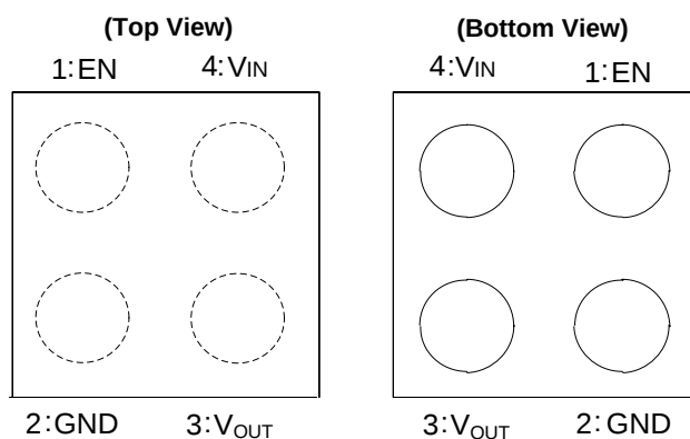
X2-WLB0606-4
