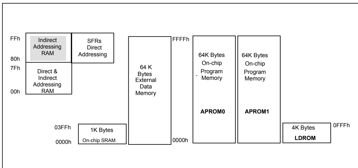
Figure 1. Memory Map
