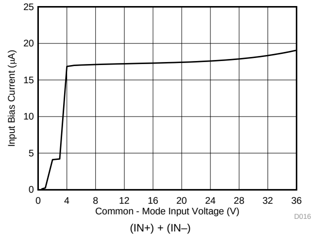
图 16. Input Bias Current vs Common-Mode Voltage
