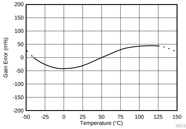
图 13. Power Gain Error vs Temperature
