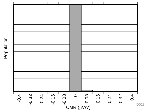
图 14. Input Common-Mode Rejection Distribution
