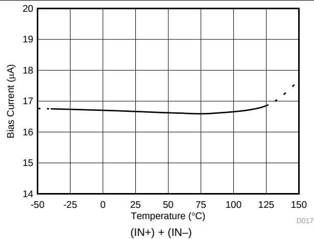
图 17. Input Bias Current vs Temperature
