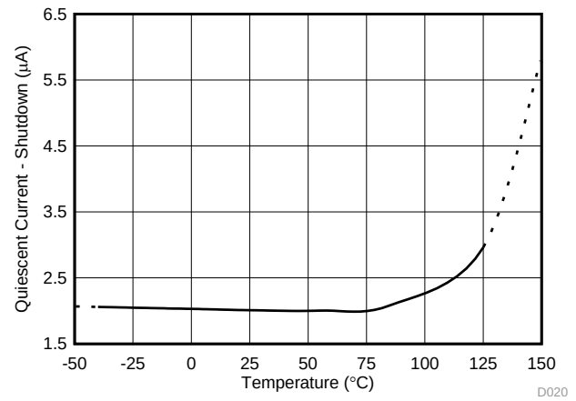
图 20. Shutdown I_Q vs Temperature
