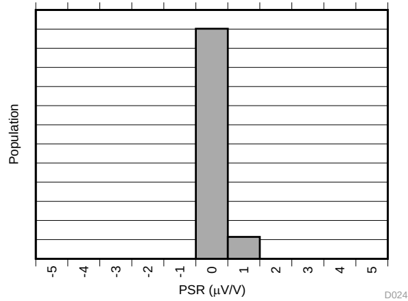
图 15. Power-Supply Rejection Distribution
