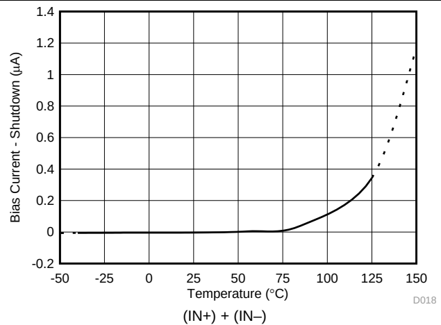
图 18. Input Bias Shutdown Current vs Temperature
