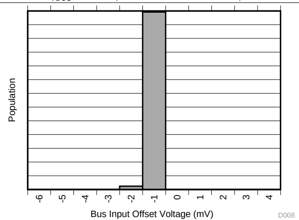
图 8. Bus Input Offset Voltage Production Distribution
