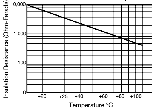
Insulation Resistance vs Temperature
