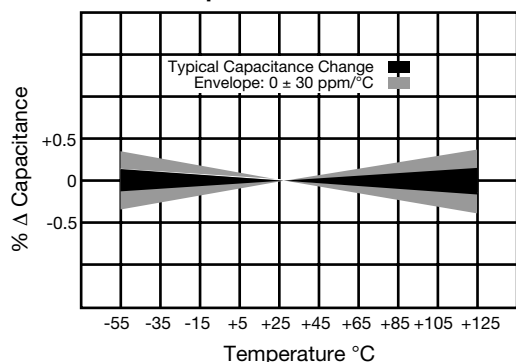
Temperature Coefficient
