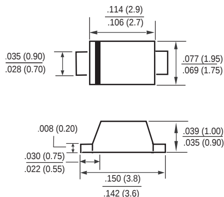
SOD-123FL
