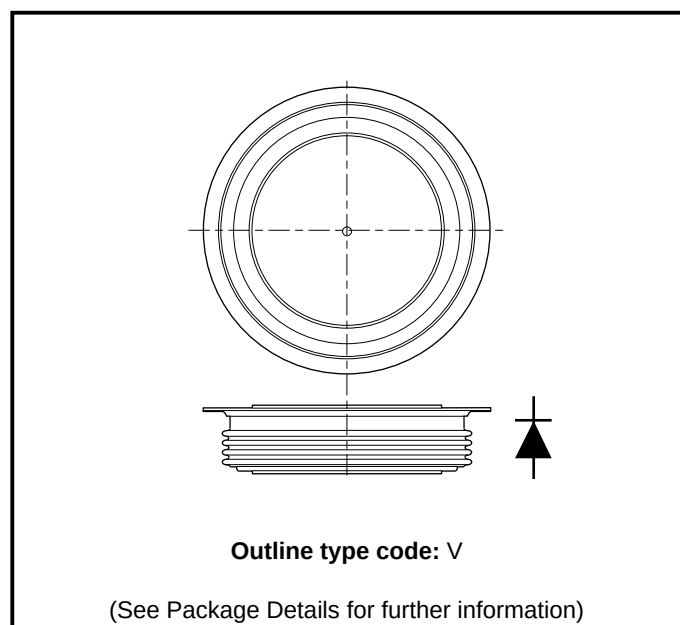
Fig. 1 Package outline
