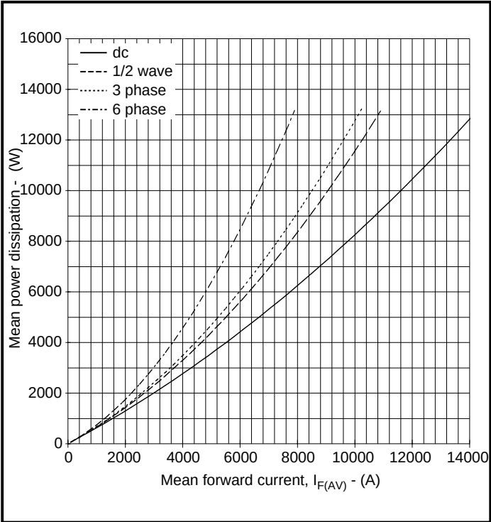
Fig. 3 Power dissipation
