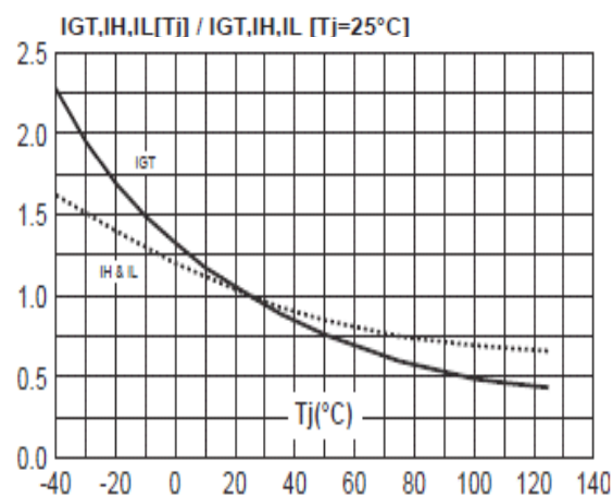
Fig.6 Relative variation of gate trigger current, holding current and latching current versus junction temperature (typical values).
