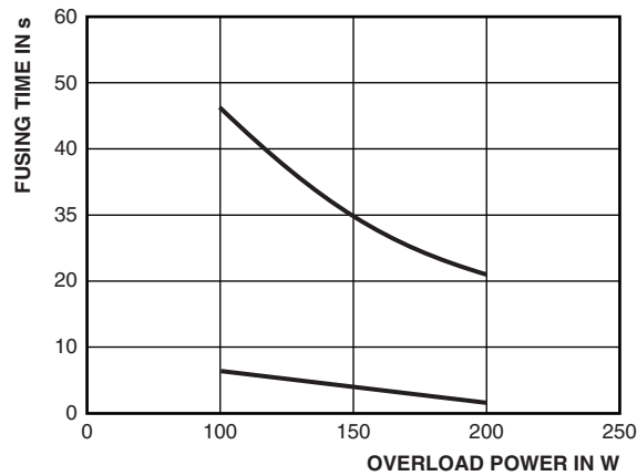
FUSING CHARACTERISTICS OF AC05-CS: 10 Ω ≤ R ≤ 100 Ω
