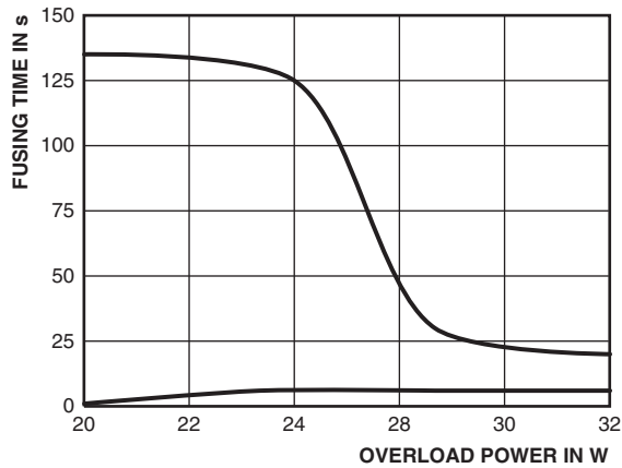
FUSING CHARACTERISTICS OF AC01-CS: 3.0 Ω ≤ R ≤ 100 Ω
