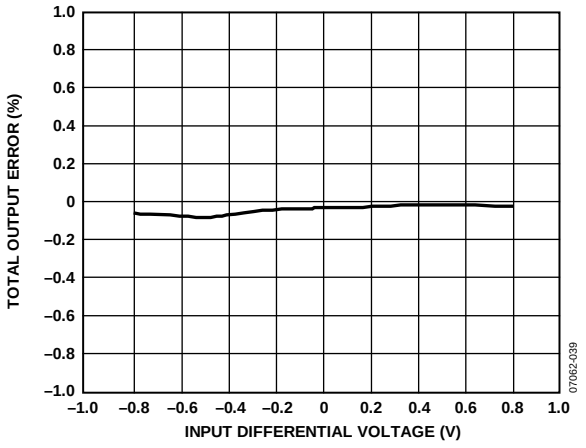
Figure 18. Output Error (%) vs. Differential Input Voltage (Bidirectional Operation ( V_{\text{REF}1} and V_{\text{REF}2} Connected to 2.5 V))
