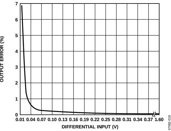
Figure 17. Output Error (%) vs. Differential Input Voltage (Unidirectional Operation ( V_{\text{REF}1} and V_{\text{REF}2} Connected to GND))
