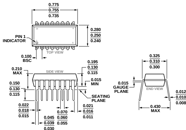
Figure 14. 16-Lead Plastic Dual In-Line Package [PDIP]
