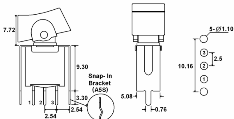
A5 (A5S – Snap-in Bracket) = PC Pins with Support Bracket (SPDT)
