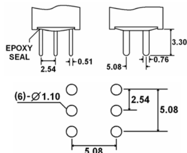
D – DPDT
