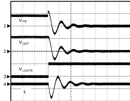
Over-Voltage-Protection
