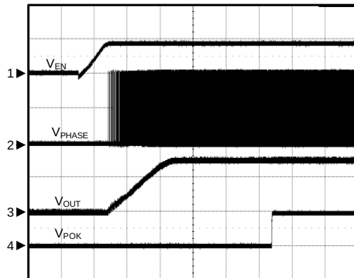
Enable(Forced PWM)
