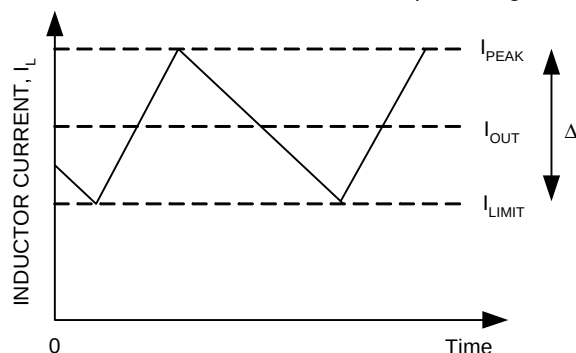
Figure 2. Current-Limit Algorithm
