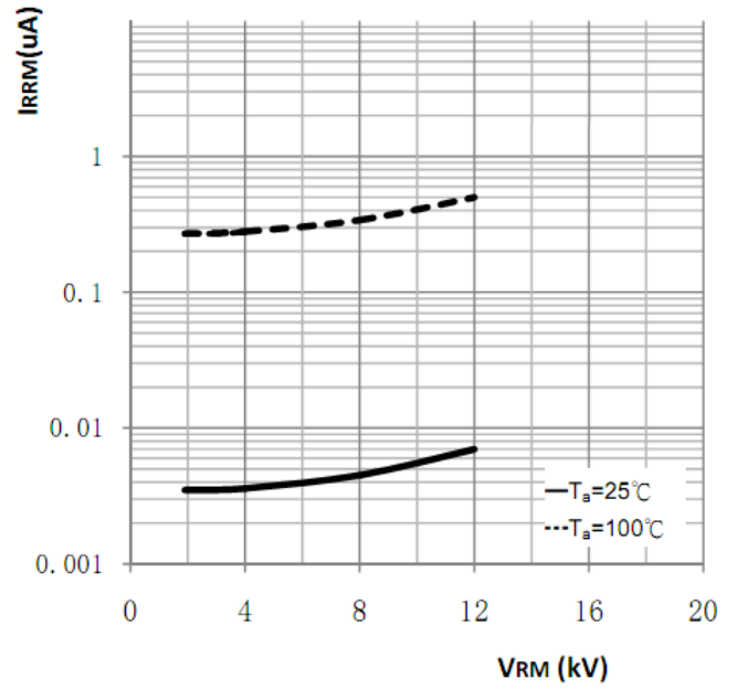
Fig2 Reverse Characteristics
