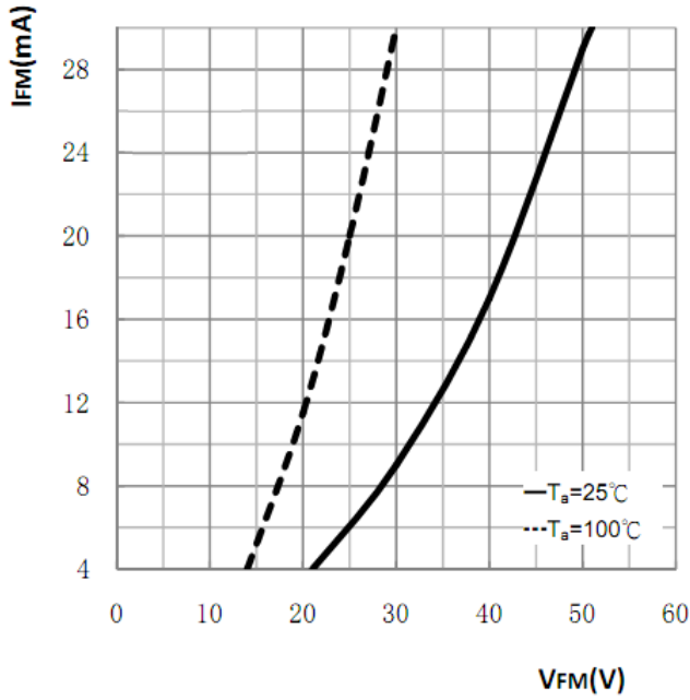
Fig1 Forward Characteristics
