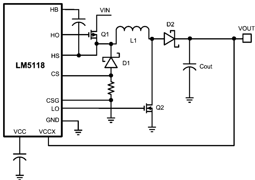
FIGURE 16. VCC Bias from VOUT 4V &lt; VOUT &lt; 15V
