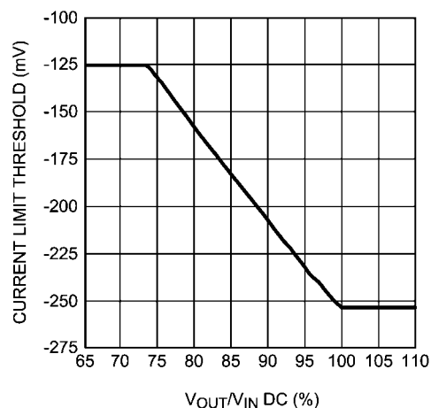
Current Limit Threshold vs VOUT/VIN VOUT = 12V
