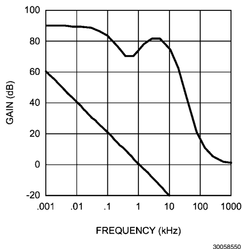
FIGURE 15. Overall Loop Gain and Phase
