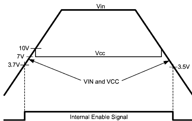
FIGURE 6. VIN and VCC Sequencing
