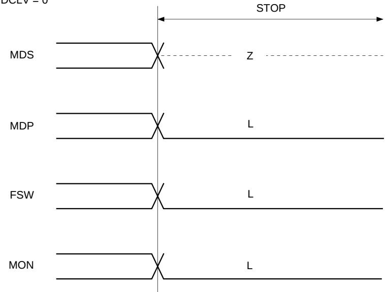
Timing Chart 1-7
