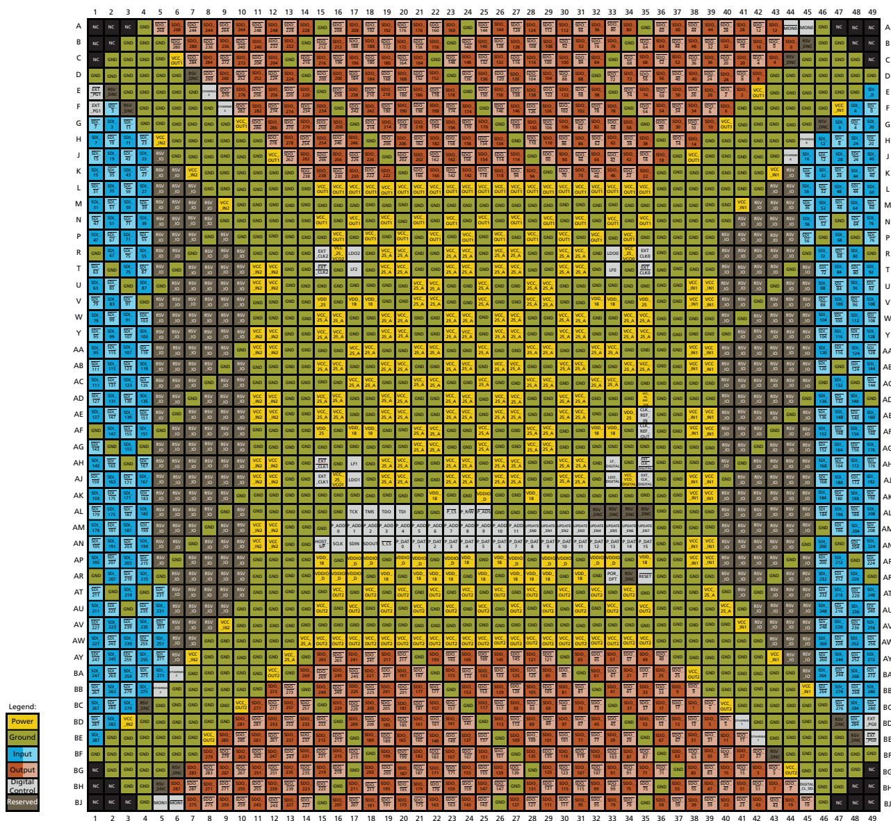
Figure 1-1: GX3190 Ball Assignment Overview (Top View)
