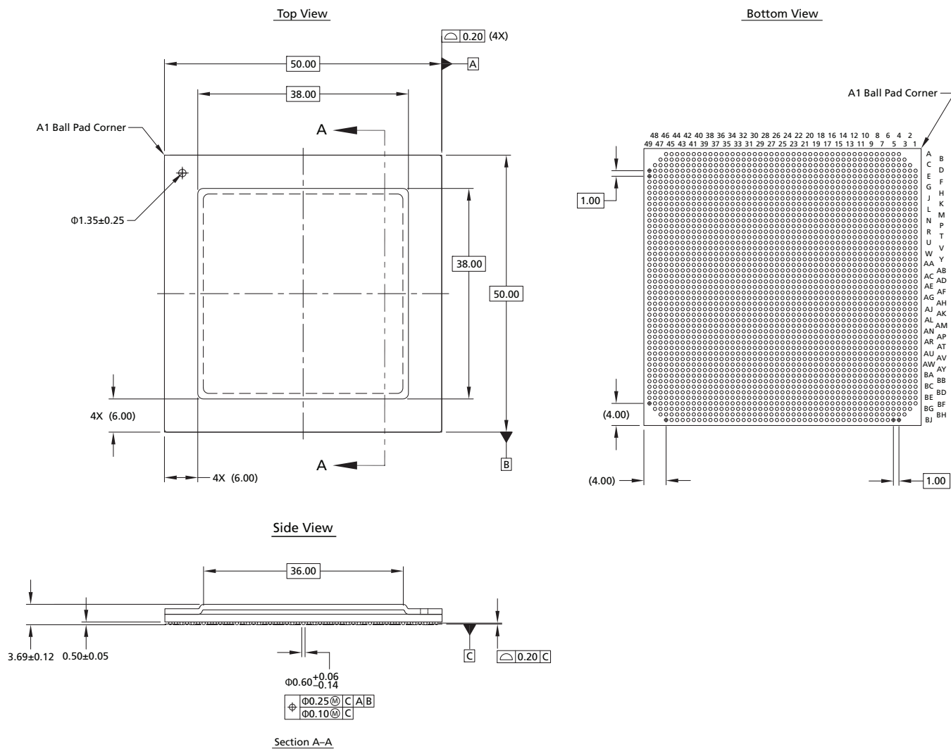
Figure 6-1: Package Dimensions
