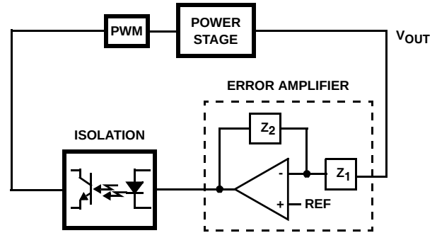
FIGURE 19. CONTROL LOOP BLOCK DIAGRAM
