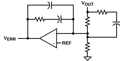
FIGURE 20. TYPE 3 ERROR AMPLIFIER
