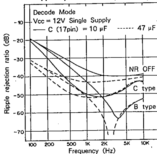
Ripple rejection ratio-4 (CXA1331)
