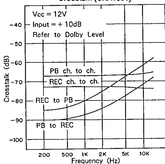
Crosstalk (CXA1331)
