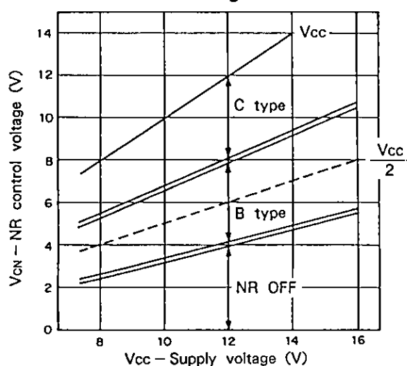
NR control voltage threshold
