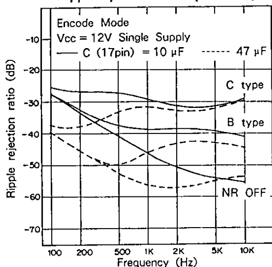
Ripple rejection ratio-3 (CXA1331)
