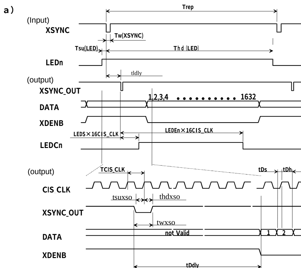
Fig. 2 Timing conditions
