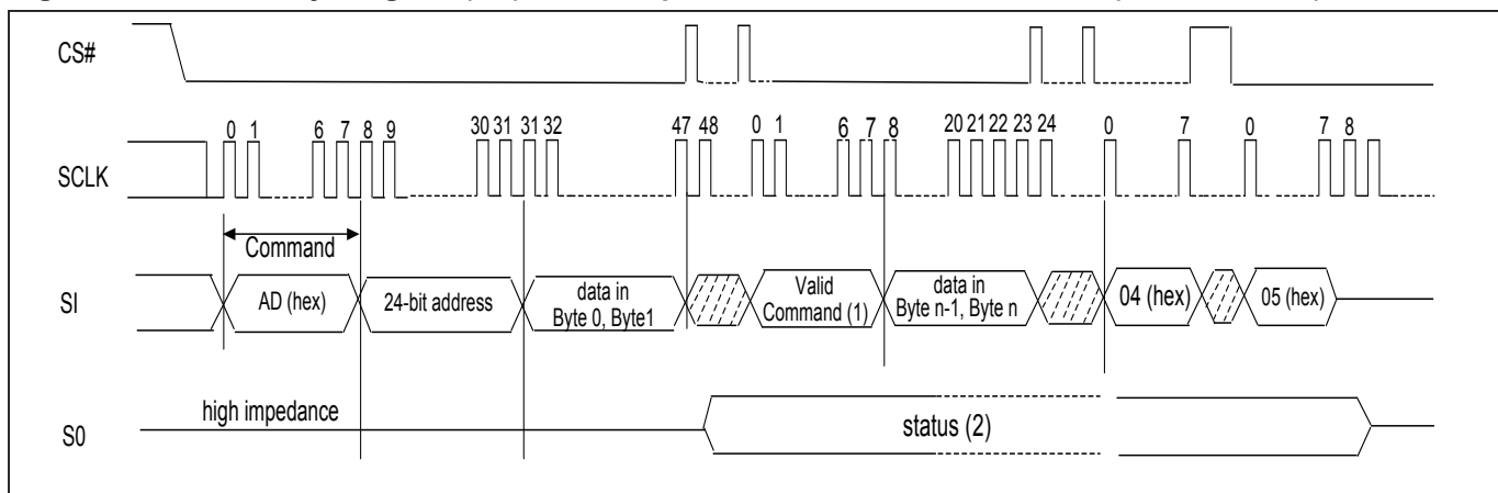
Figure 22. Continously Program (CP) Mode Sequence with Hardware Detection (Command AD)
