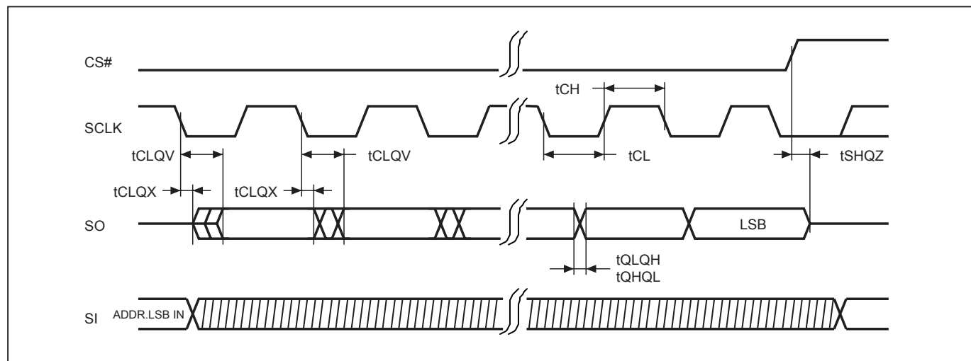
Figure 7. Output Timing
