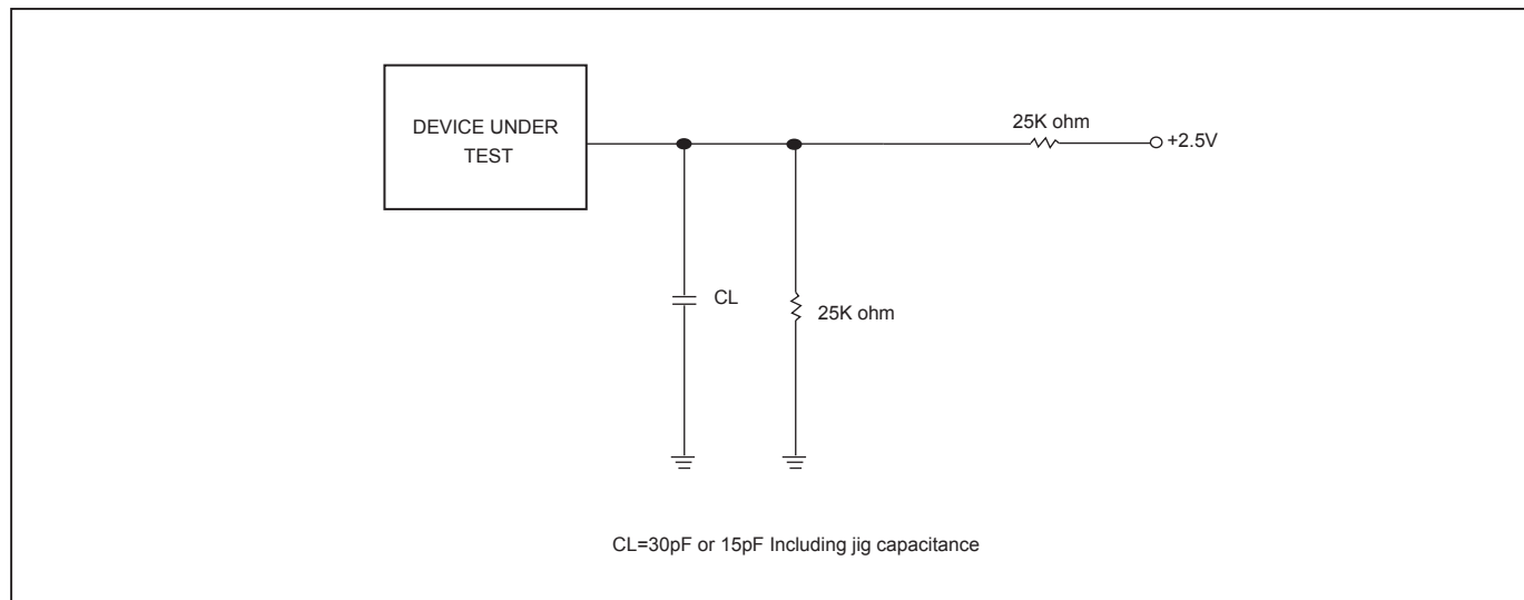
Figure 5. OUTPUT LOADING
