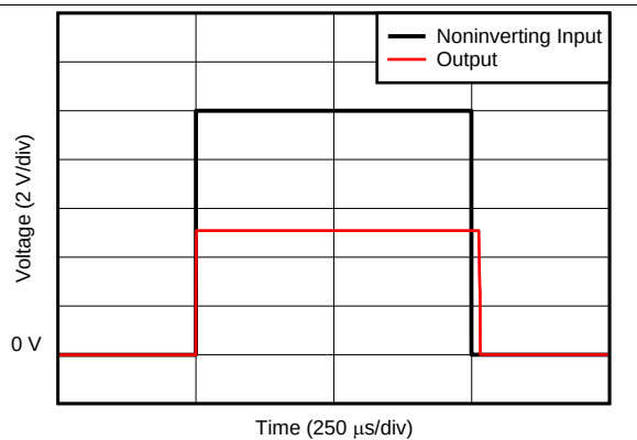
Figure 32. Common-Mode Voltage Transient Response
