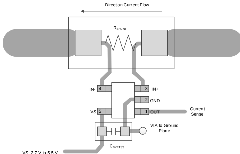
Figure 51. Single-Channel Recommended Layout (Pinout A)
