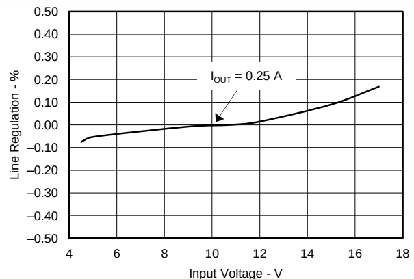
Figure 11. Line Regulation
