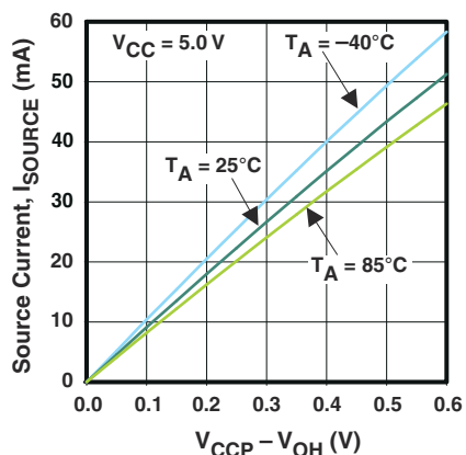
图 6-15. I/O Source Current vs Output High Voltage
