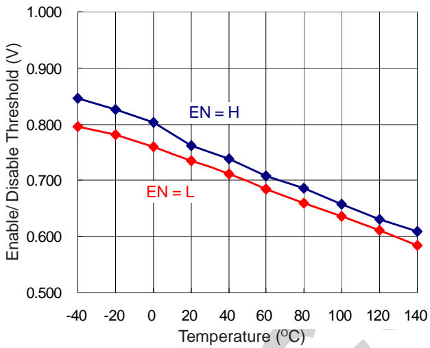
Enable/ Disable Threshold vs. Temperature
