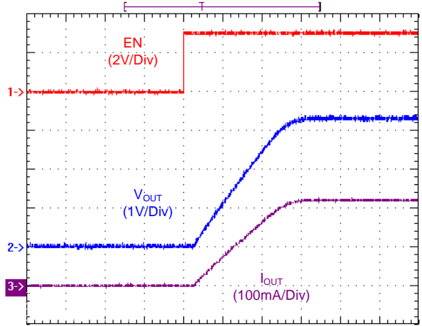
Turn On Waveform
