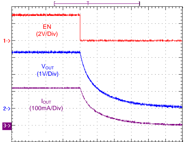
Turn Off Waveform
