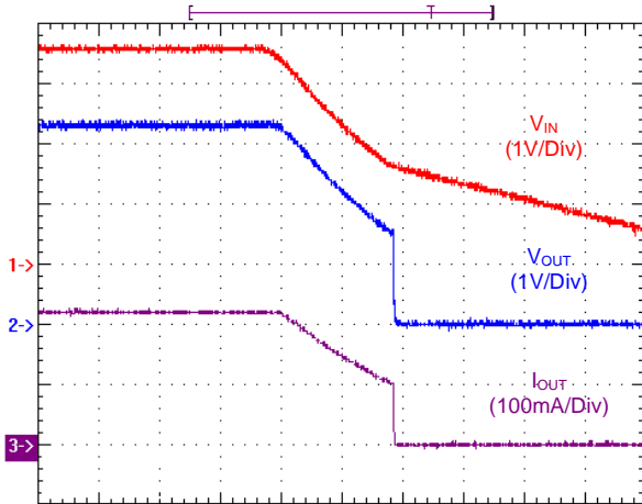
Power Off Waveform
