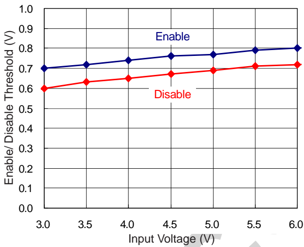
Enable/ Disable Threshold vs. Input Voltage
