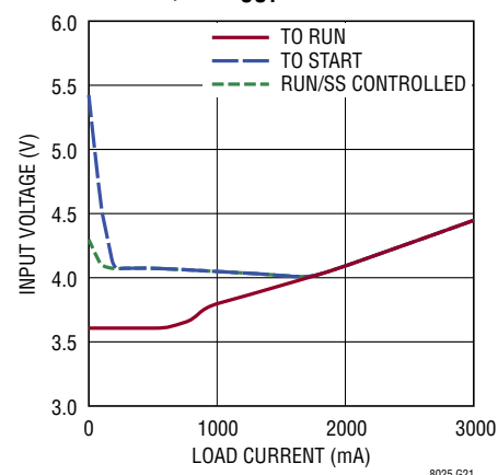
Minimum Input Voltage vs Load Current, 3.3V_{OUT}
