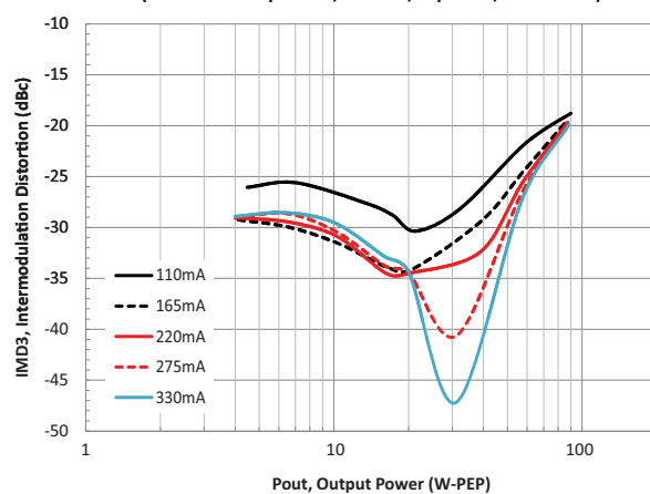
IMD3 vs. Pout (2-Tone 1MHz Separation, Vd = 48V, Idq varied, fc = 900MHz)
