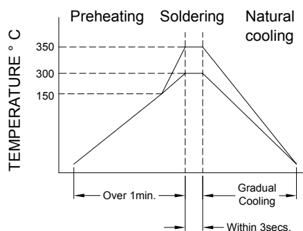
Figure 2. Iron Soldering
