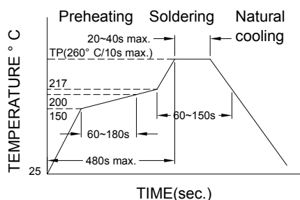
Figure 1. Re-flow Soldering
