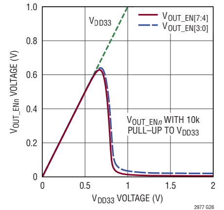
V OUT_EN[7:0] Output Voltage vs V DD33
