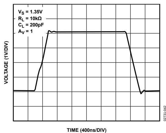
Figure 42. Large Signal Transient Response
