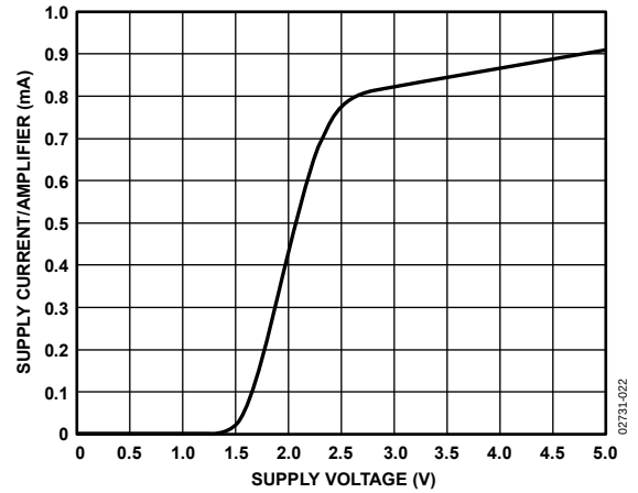
Figure 22. Supply Current/Amplifier vs. Supply Voltage
