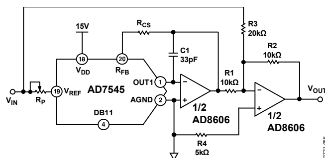
Figure 56. Bipolar Operation
