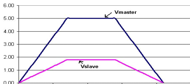
Figure 13. Ratiometric Tracking Plot
